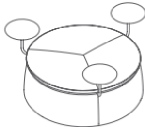
LAS3STAB Lasso 3 Seat Stool and Tables mm W 1425 D 1465 H 705 Seat 485 inch W 56 D 57.5 H 28 Seat 19
